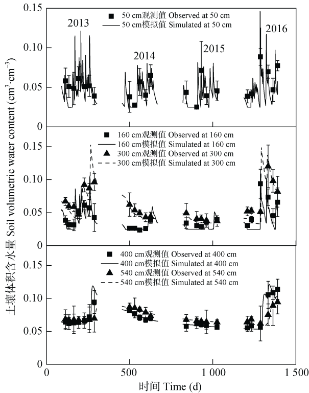
图 3 2013—2016 年六道河流域不同深度土壤体积含水量实测值与模拟值随时间变化对比 Fig. 3 Comparison between dynamic changes of the observed and simulated soil volumetric water contents at different depths at the Liudaogou catchment in 2013–2016
